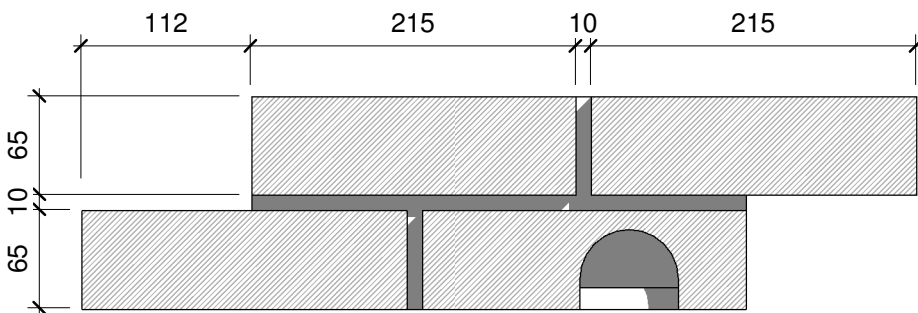
Front Elevation
