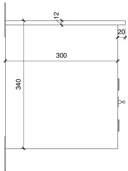
Side Elevation
