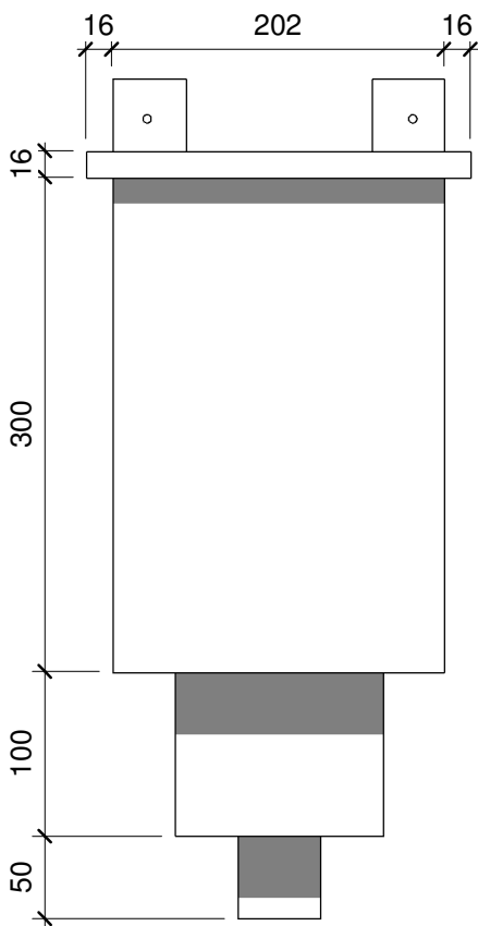
Front Elevation
