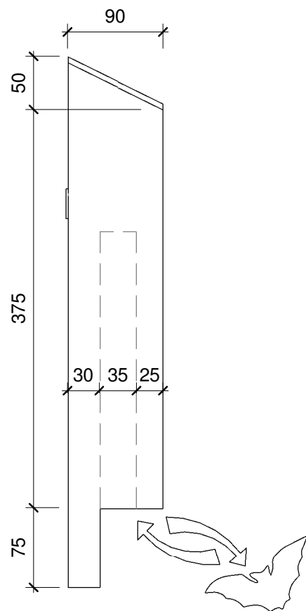
Side Elevation
